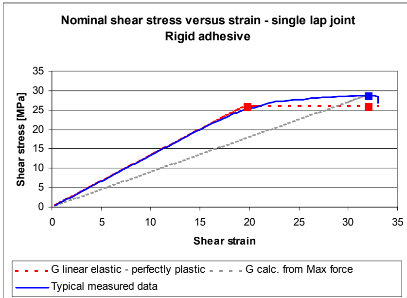
Material models for rigid adhesives
