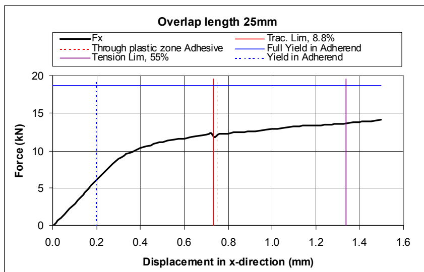
Test results, overlap joint versus FEM analysis design limits for adhesive and adherends
