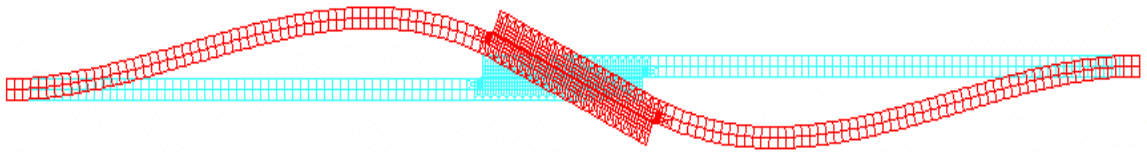
FEM analysis - initial and deformed shape of single lap bonded joint in tension
