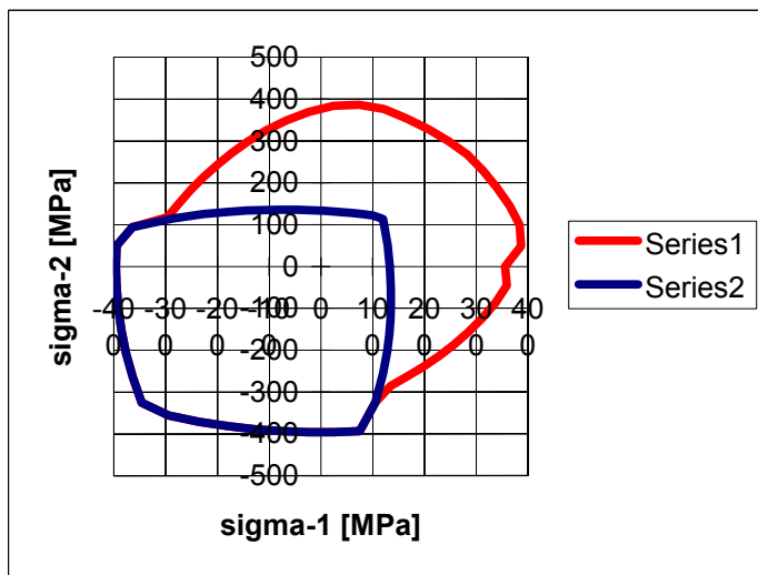
Failure envelope of 0/90 laminate, combined in-plane loading
