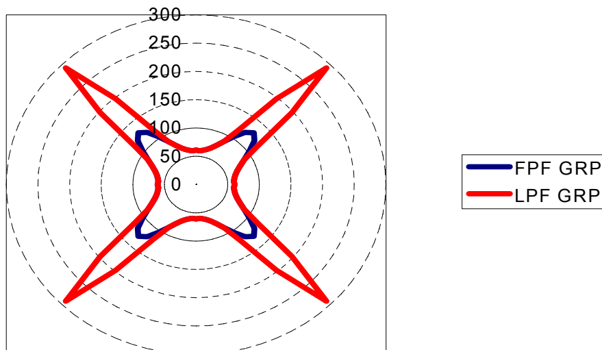
Direction dependency of shear load on a \pm 45^\circ laminate
