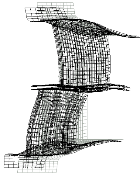
Deformed shape (exaggerated)
