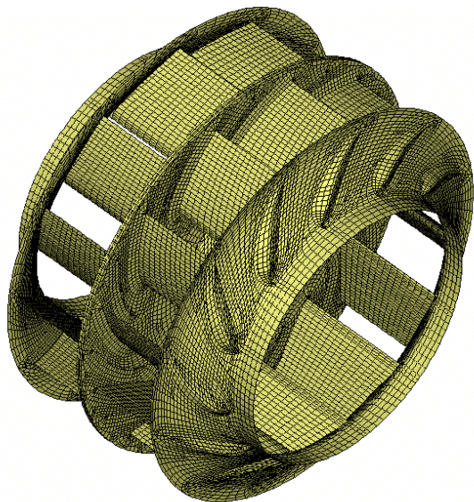
FE-model used for analyses
