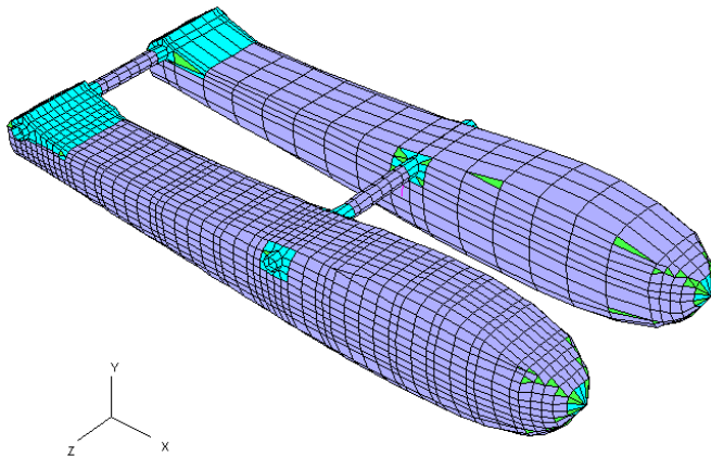
FE-model(MAESTRO) used for analyses
