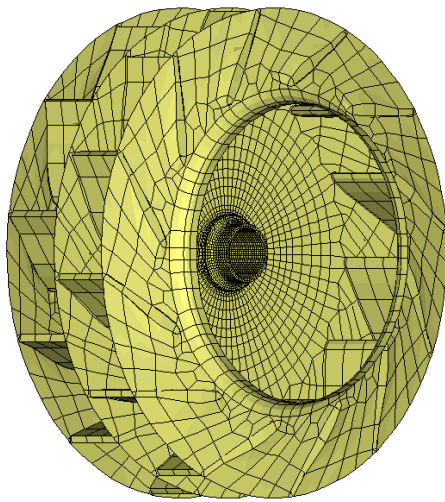
FE-model used for analyses
