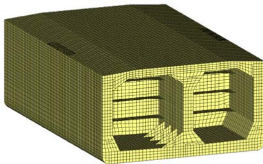
FE-model ship module
