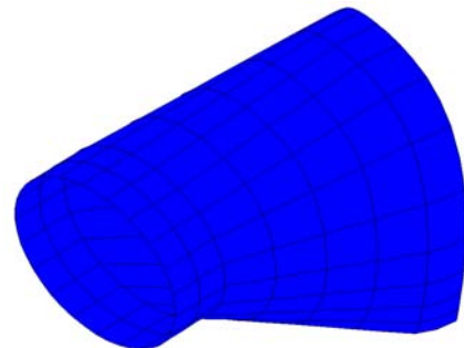
FE-model of boss
