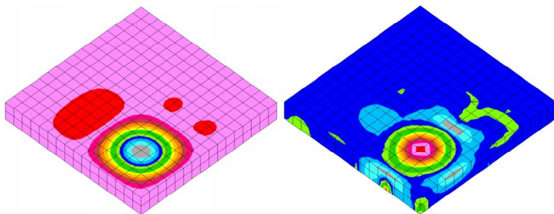
Deformation and stress plot form analyses of mock up
