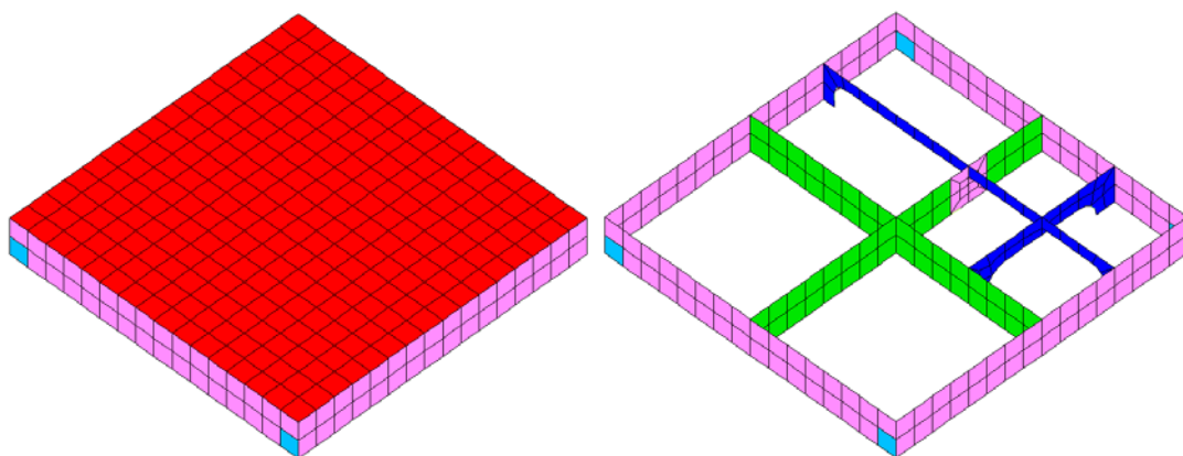
FE-model of mock up
