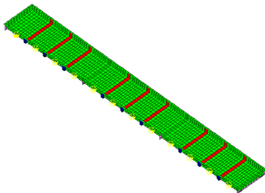
FEM model with boundary conditions
