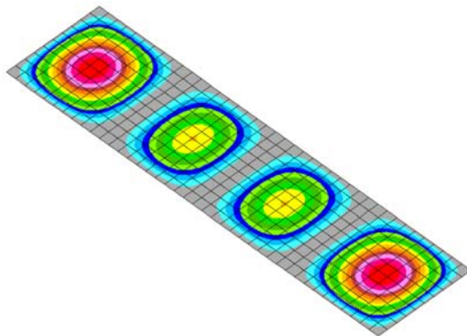
FE-model showing flooring deformation
